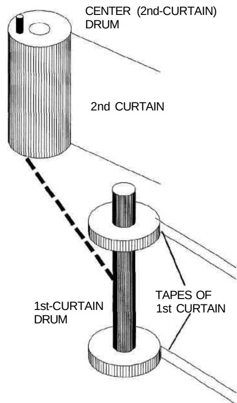
FIG. FP8 Construction of the curtain drum.
