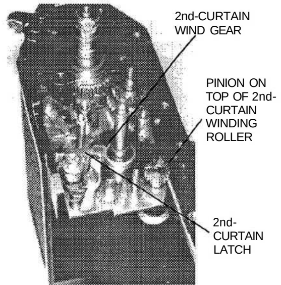
FIG. FP39 Adjusting the timing of the 2nd curtain.
