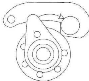
FIG. FP19 2nd-curtain release lever set to fastest shutter speed.
