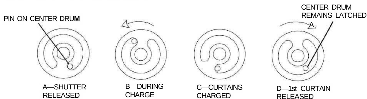
FIG. FP10 Top section of 1st-curtain drum.
