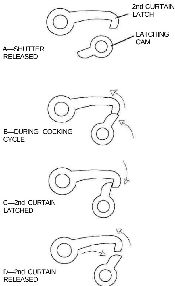
FIG. FP16 Latching sequence for 2nd-curtain winding roller.
