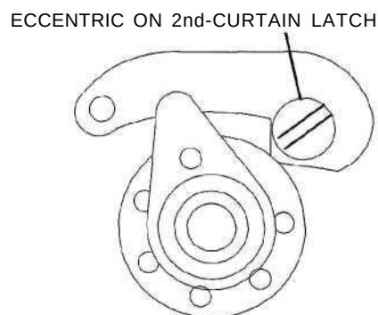
FIG. FP28 Top of drum-type focal-plane shutter.
