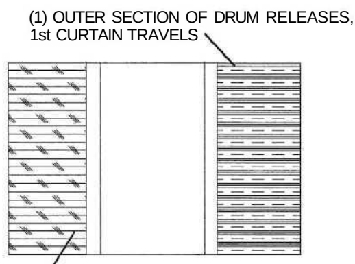
FIG. FP11 Curtains viewed from front of camera.
