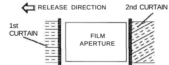
C—1st CURTAIN RELEASED, 2nd CURTAIN LATCHED
